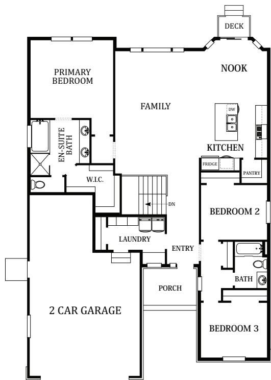
MAIN FLOOR
