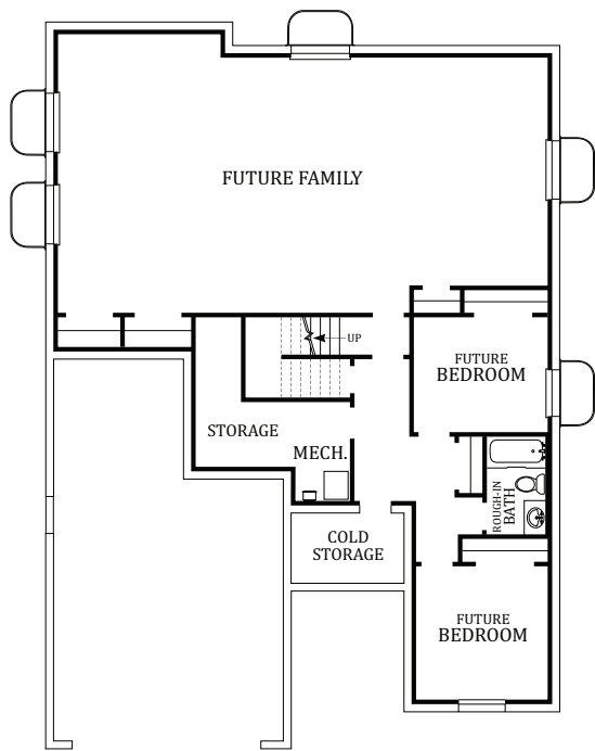
BASEMENT
