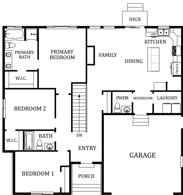
MAIN FLOOR
