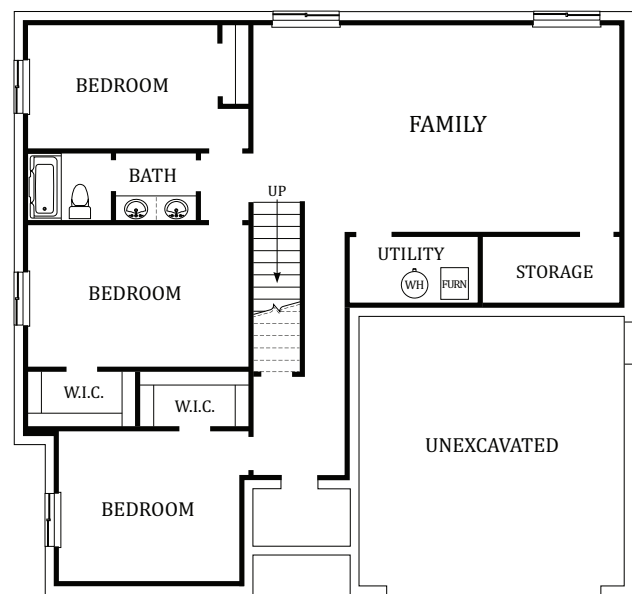
BASEMENT
