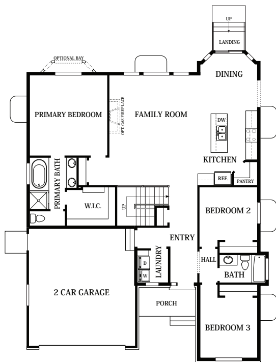
MAIN FLOOR
