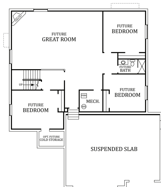
BASEMENT
