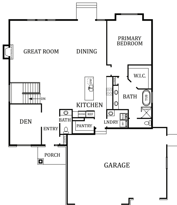
MAIN FLOOR
