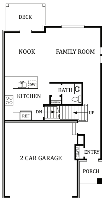
MAIN FLOOR
