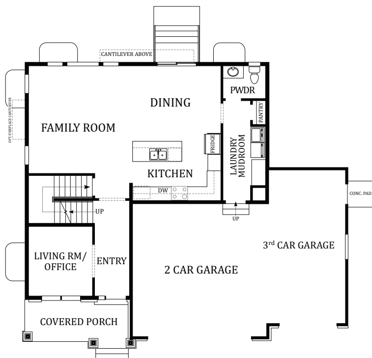
MAIN FLOOR
