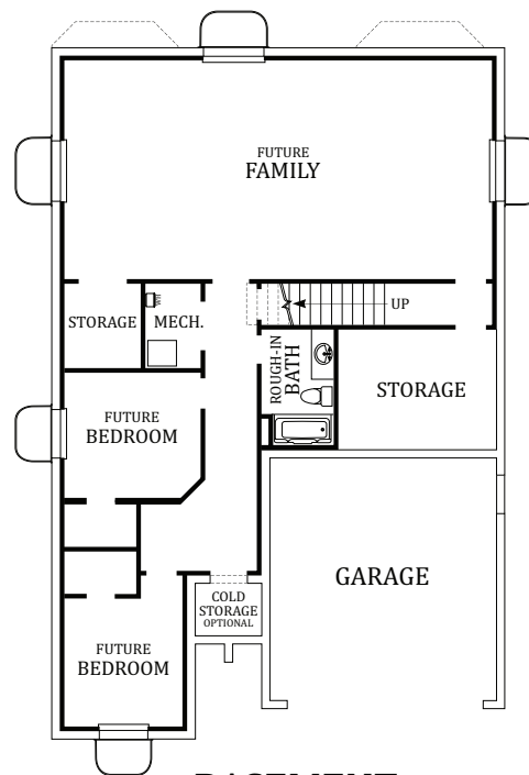
BASEMENT
