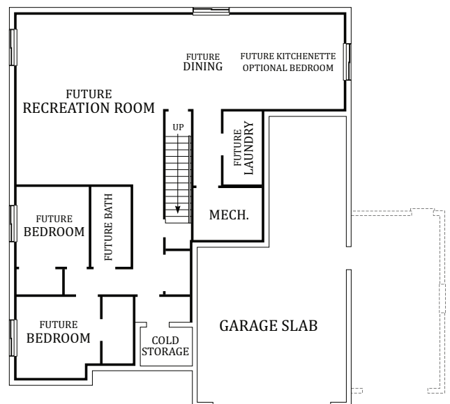
FUTURE BASEMENT FLOOR PLAN
