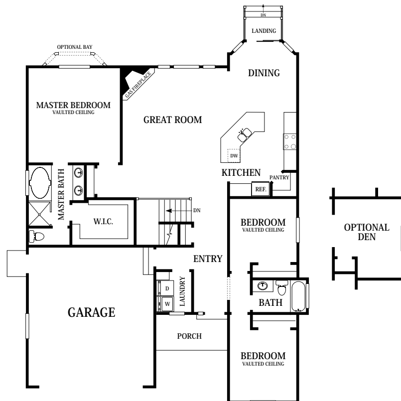
MAIN FLOOR
