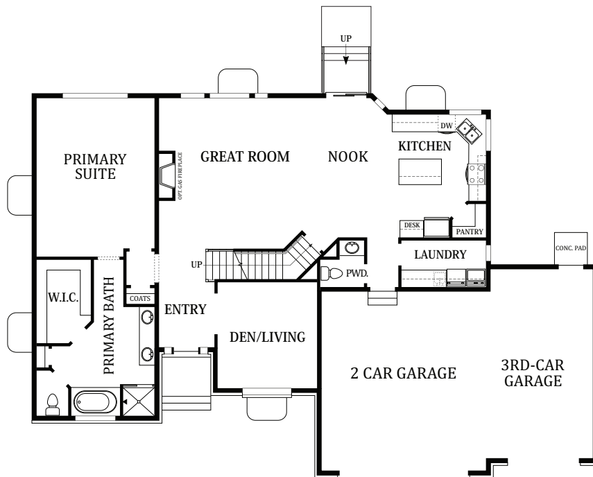
MAIN FLOOR
