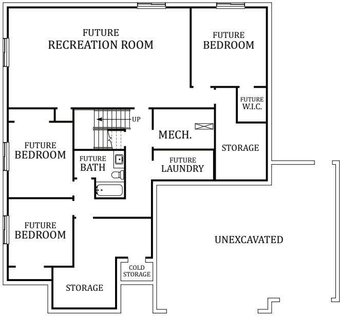
FUTURE BASEMENT
